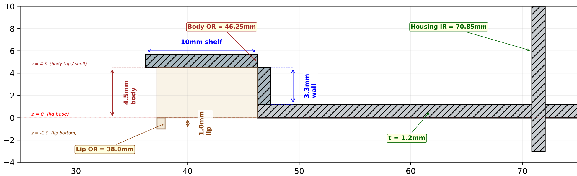
DETAIL B — Flush Ceramic Pocket (4x scale)
