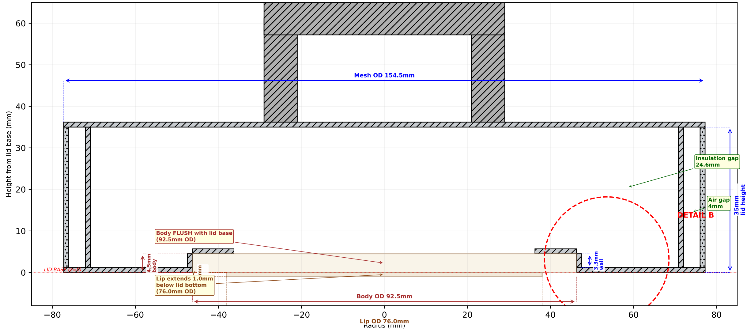
Section B-B — Ceramic flush, lip extends below
